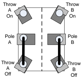
DPDT Power Switch (OFF POSITION)
