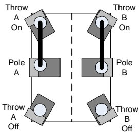
DPDT Power Switch (ON POSITION)
